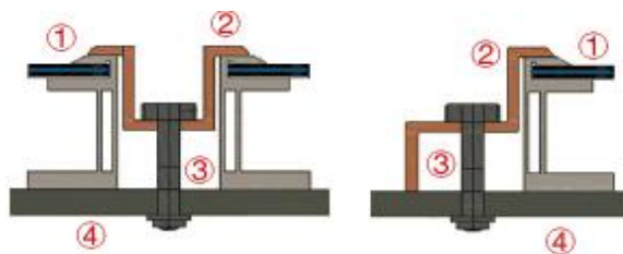
①frame ②Clip ③M8 bolt ④ mounting rail
